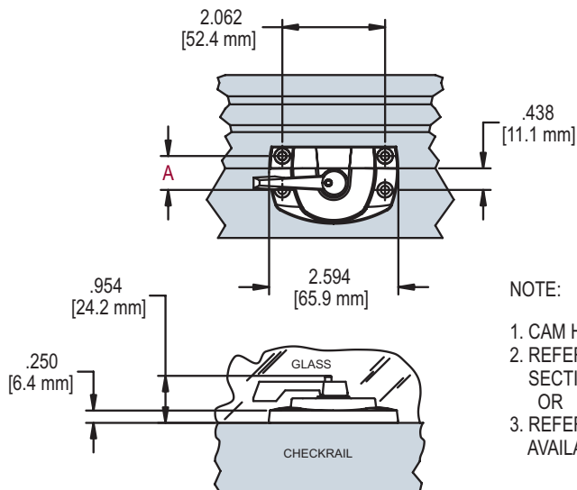
FIG. 2 APPLICATION OF TRUTH ENTRYGARD* II BUTTON LOCK
