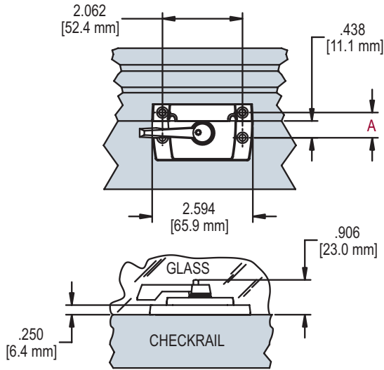
FIG. 1 APPLICATION OF TRUTH TRIMLINE BUTTON LOCK
