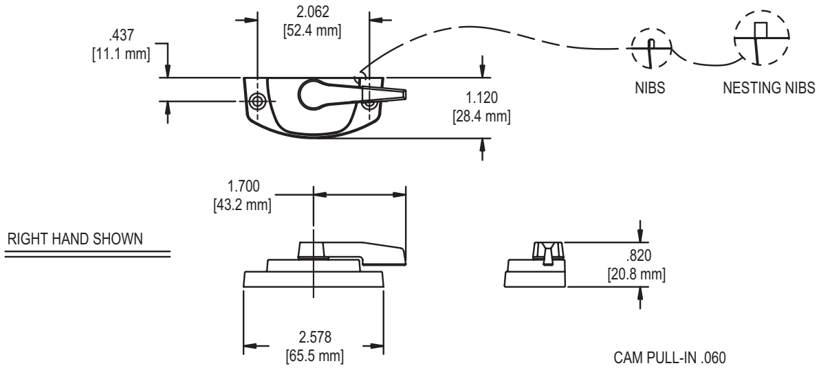
FIG. 1 SASH LOCK AND KEEPER
